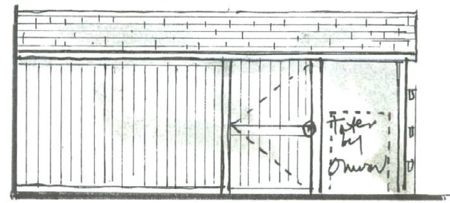
Front Elevation Storage / Tool Shed
